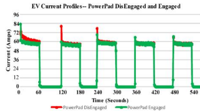
PowerPad Current Performance DisEngaged and Engaged
