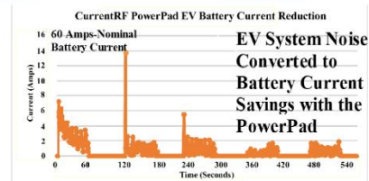
EV Battery Current Reduction From EV Noise
