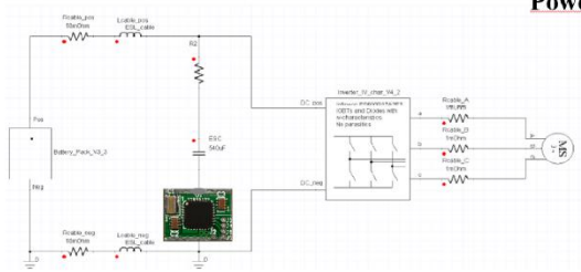
PowerPad Insertion on the Ground Side of a DC-Link Capacitor
