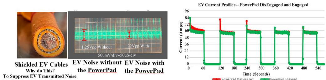
PowerPad Current Performance DisEngaged and Engaged
